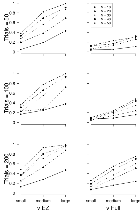
Figure 5. Proportion of times a significant between-group effect was detected with the diffusion model drift rate estimates. Left column = EZ diffusion \nu ; right column = full diffusion \nu . Top row = 50 trials, middle row = 100 trials, bottom row = 200 trials. Different lines indicate different numbers of participants per group.
