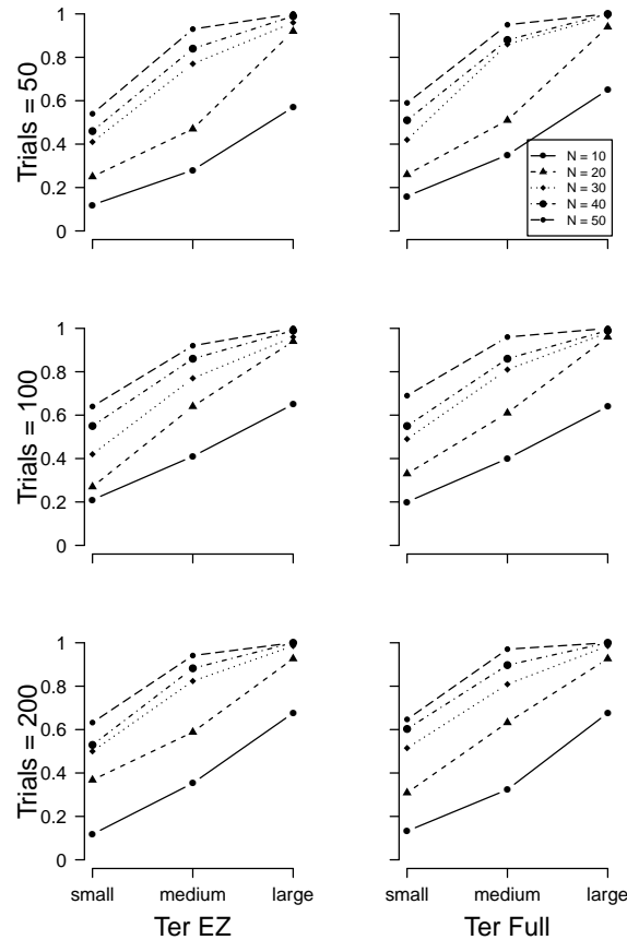
Figure 4. Proportion of times a significant between-group effect was detected with the diffusion model non-decision time estimates. Left column = EZ diffusion T_{er} ; right column = full diffusion T_{er} . Top row = 50 trials, middle row = 100 trials, bottom row = 200 trials. Different lines indicate different numbers of participants per group.
