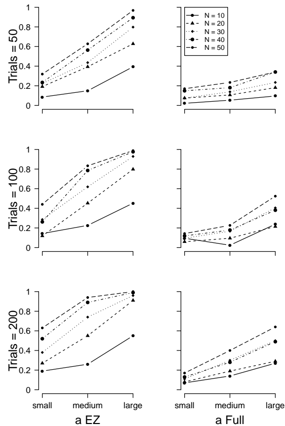
Figure 3. Proportion of times a significant between-group effect was detected with the diffusion model boundary separation estimates. Left column = EZ diffusion a ; right column = full diffusion a . Top row = 50 trials, middle row = 100 trials, bottom row = 200 trials. Different lines indicate different numbers of participants per group.
