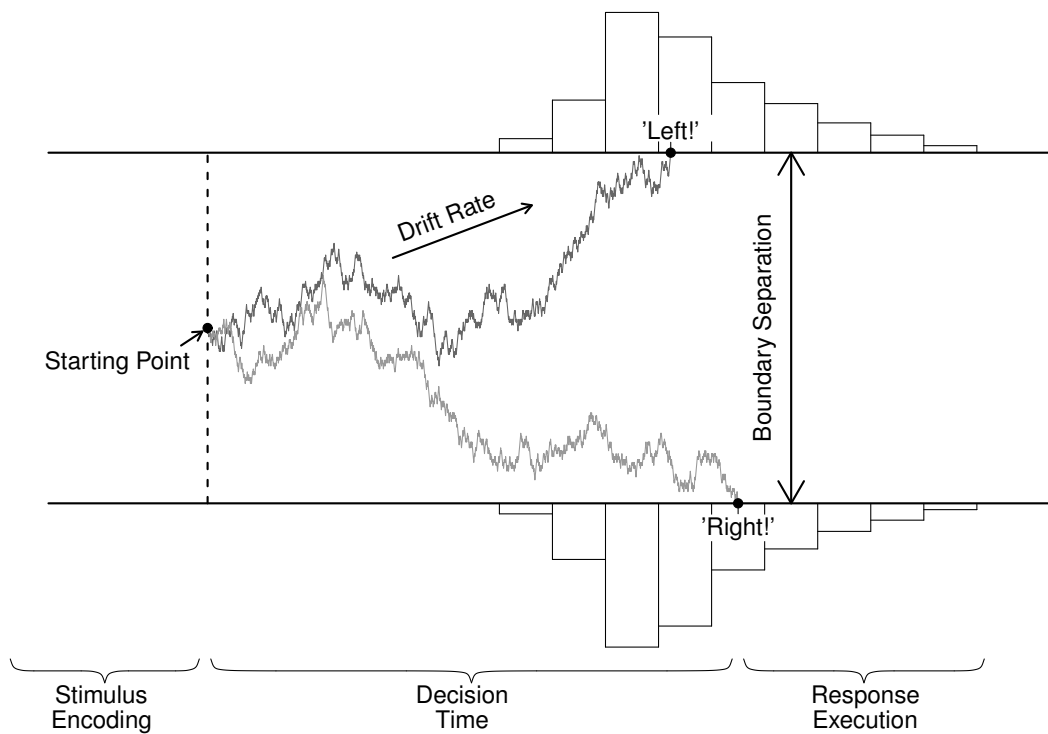
Figure 1. The diffusion model and its parameters as applied to a moving dots task (Ball & Sekuler, 1982). Evidence accumulation begins at starting point z , proceeds over time guided by mean drift rate \nu , and stops whenever the upper or the lower boundary is reached. Boundary separation a quantifies response caution. Observed RT is an additive combination of the time during which evidence is accumulated and non-decision time T_{er} .
