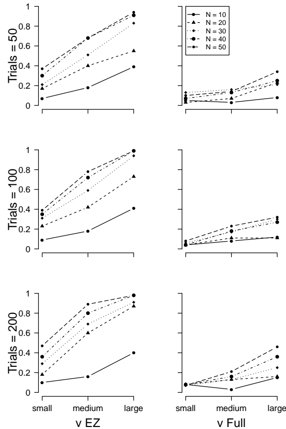
Figure 2. Proportion of times a significant between-group effect was detected with the diffusion model drift rate estimates. Left column = EZ diffusion \nu ; right column = full diffusion \nu . Top row = 50 trials, middle row = 100 trials, bottom row = 200 trials. Different lines indicate different numbers of participants per group.
